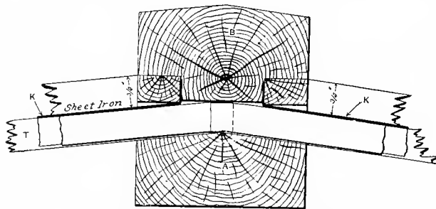
Fig. 2382. Cross Section of Ridge-pole.
